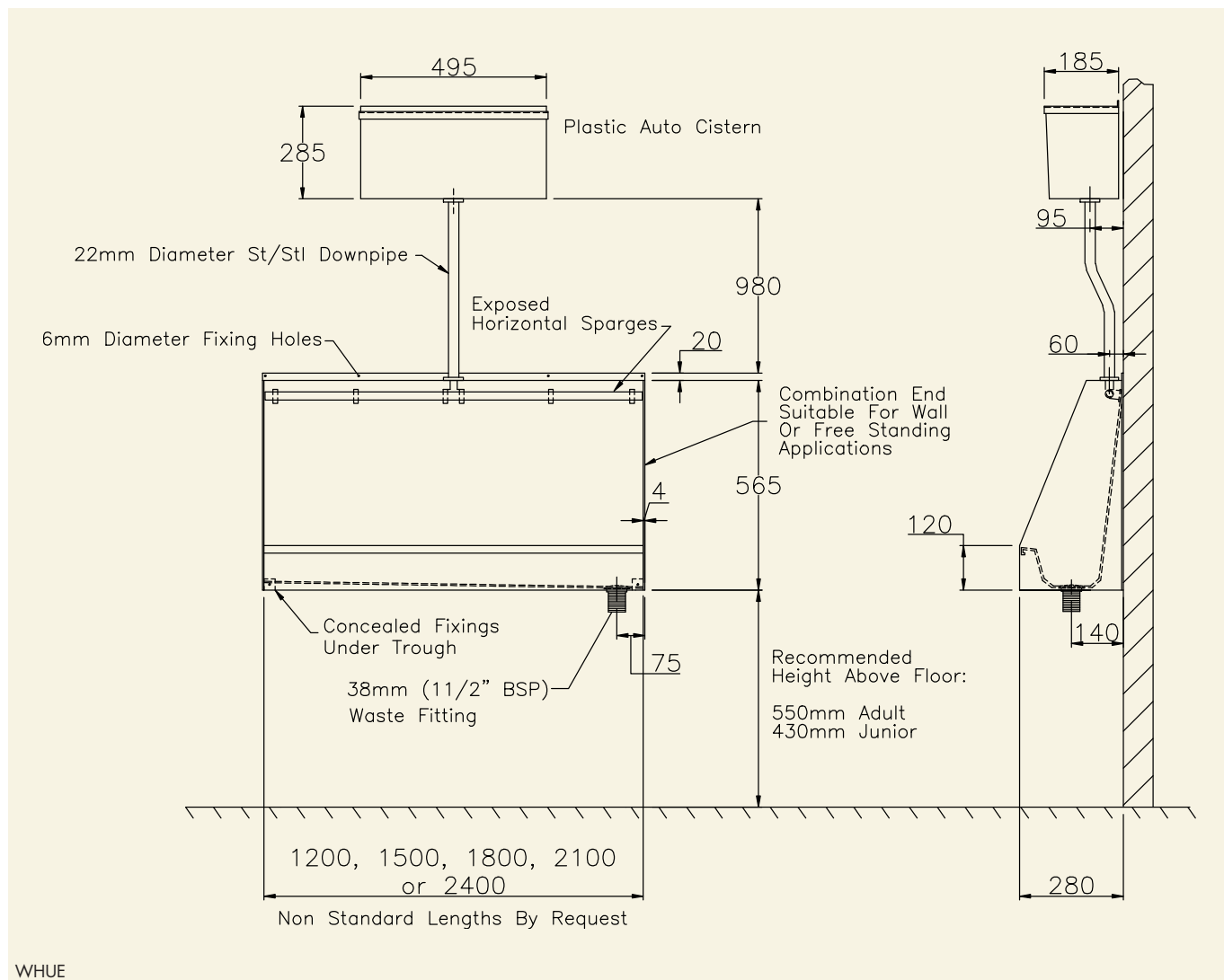
2 WHUE Plastic automatic flushing cistern
