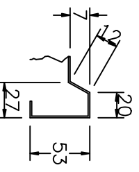
Anti Drip Edge at Drainer Ends
