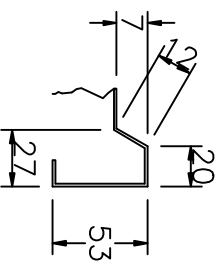
Anti Drip Edge at Drainer End
