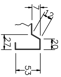
Anti Drip Edge at Drainer Ends
