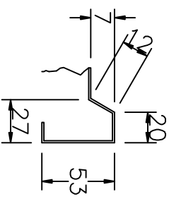
Anti Drip Edge at Drainer End
