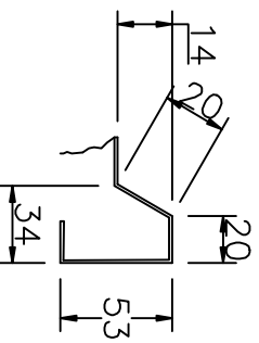
Anti Drip Edge at Bowl End
