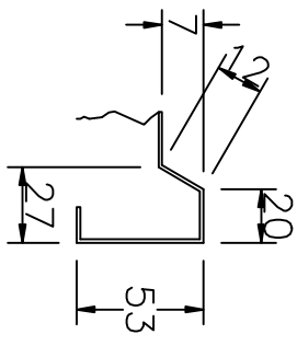
Anti Drip Edge at Drainer End
