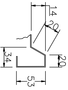
Anti Drip Edge at Bowl End
