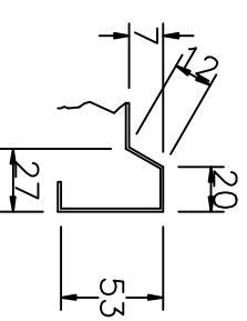
Anti Drip Edge at Drainer Ends
